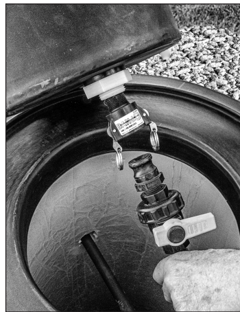
Float valve tub disconnected.
