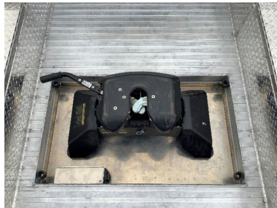
Reusing Factory 5 th wheel Puck system
